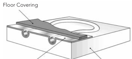
Floor Covering Aluminium Diffusion Plate Floating Floor Panel (30/40/50mm available)
