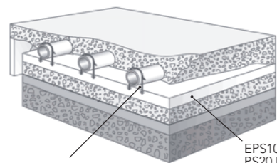
'U' Clip EPS100 PS20 Insulation (25mm or 50mm)
